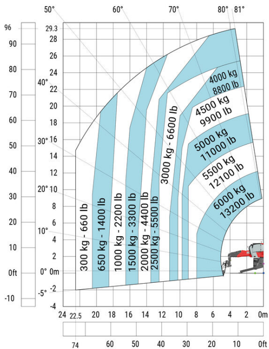
Machine on lowered stabilizers with winch 13,200 lb
