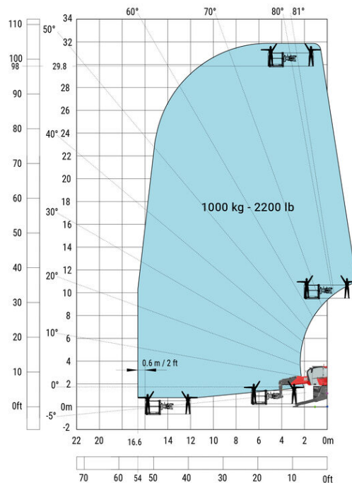
Machine on lowered stabilizers with 2,200 lb platform
